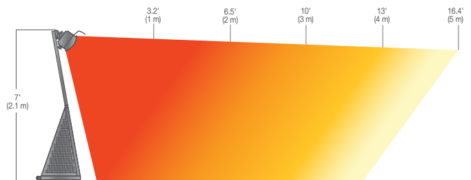
SIDE PROFILE
