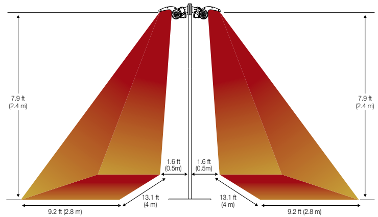
Outdoor heating area
