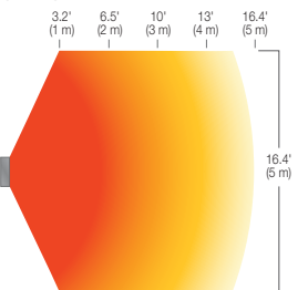
TOP PROFILE
